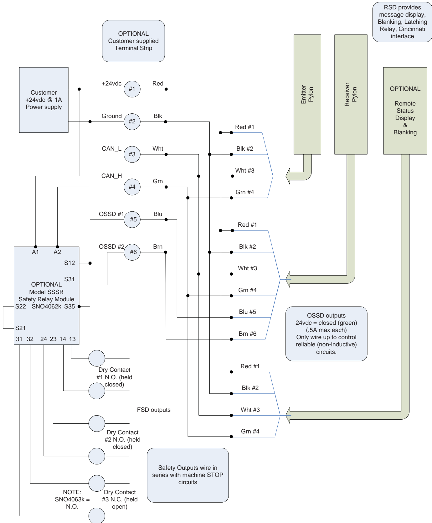
Model CA 28-142 Wiring Diagram (with EDM)
